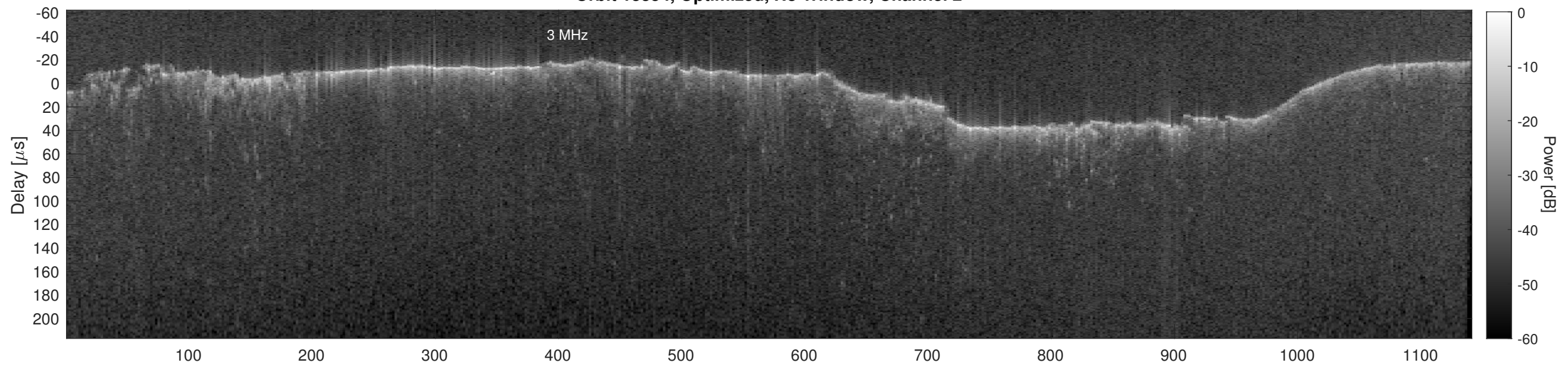
Orbit 13354, Cluttergram
