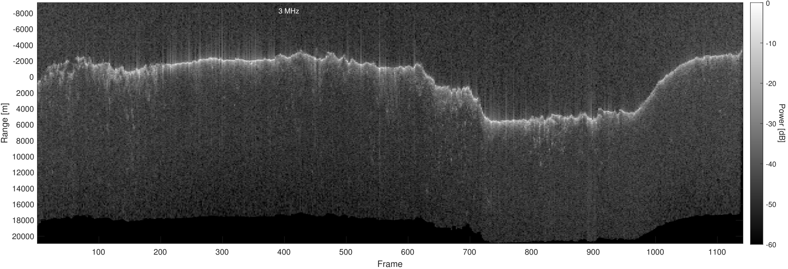
Orbit 13354, Optimized, No Window, Depth-Corrected, Channel 2
