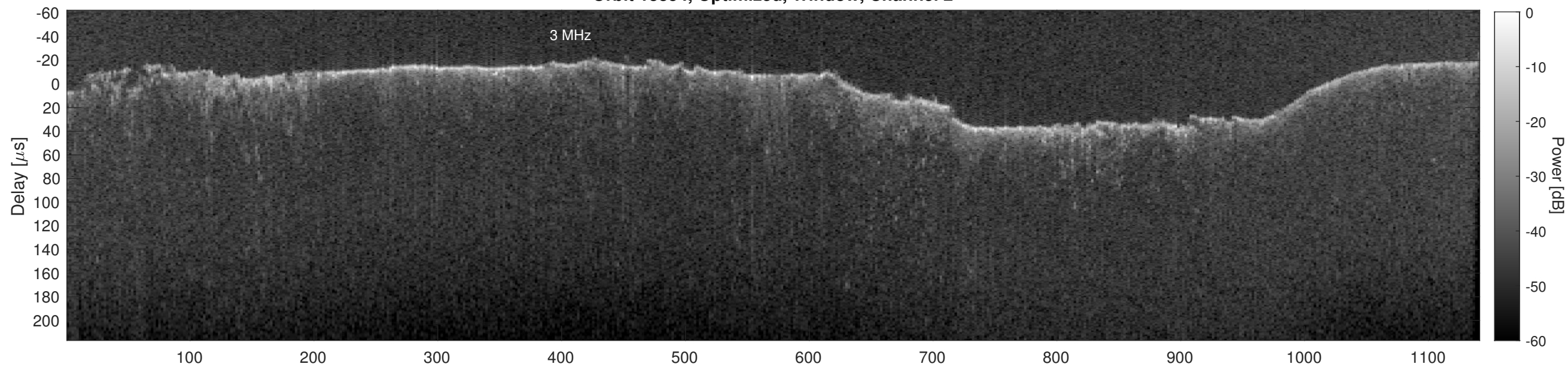
Orbit 13354, Cluttergram
