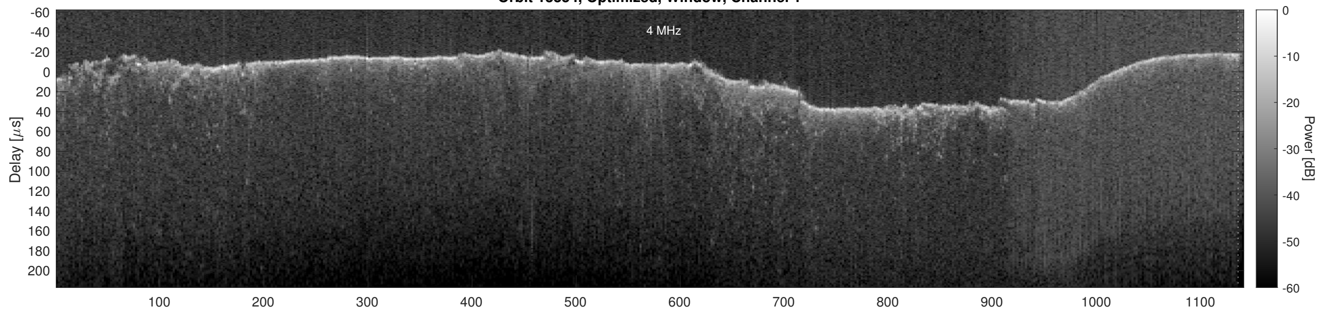
Orbit 13354, Optimized, Window, Channel 2
