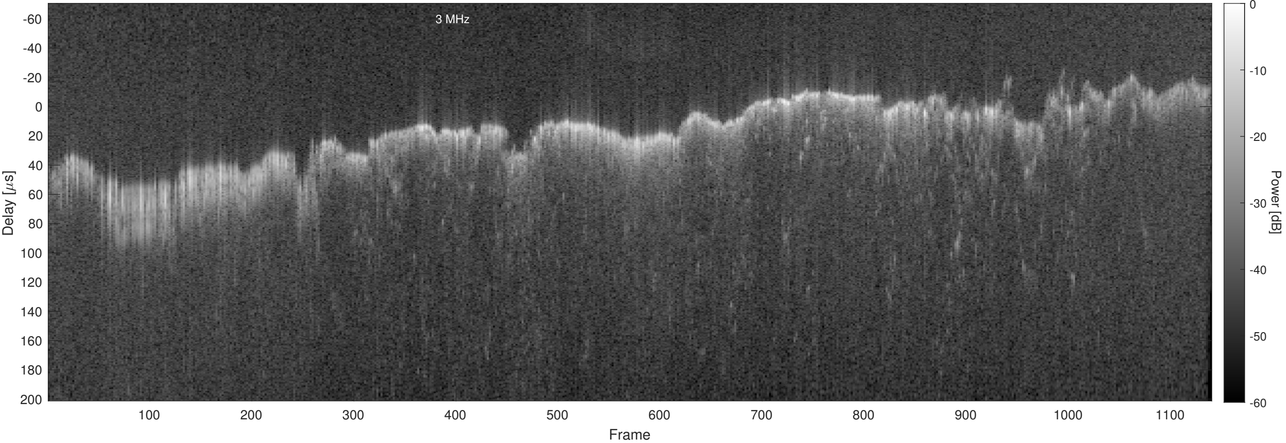
Orbit 13355, Chapman, No Window, Channel 2
