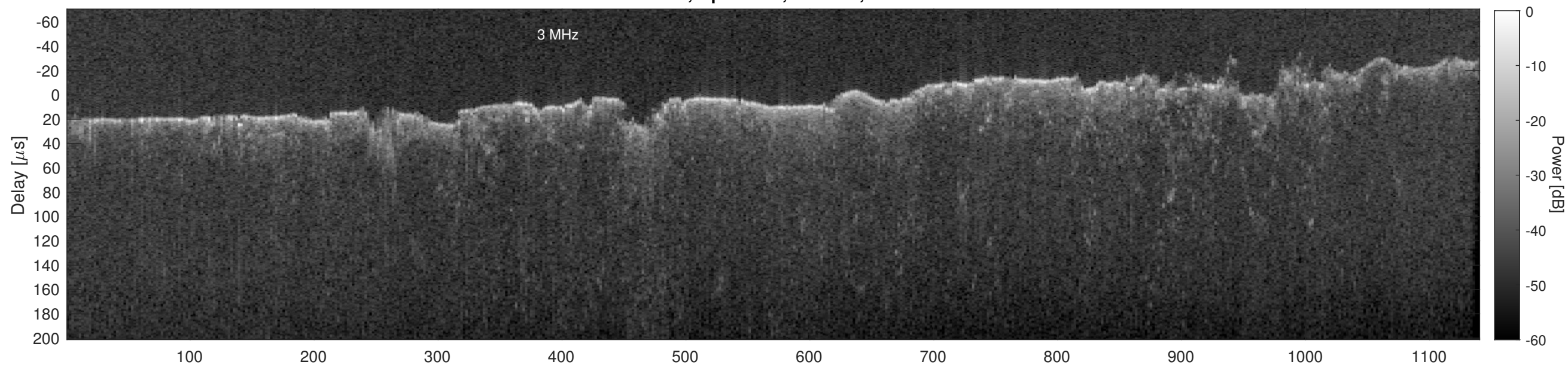
Orbit 13355, Cluttergram
