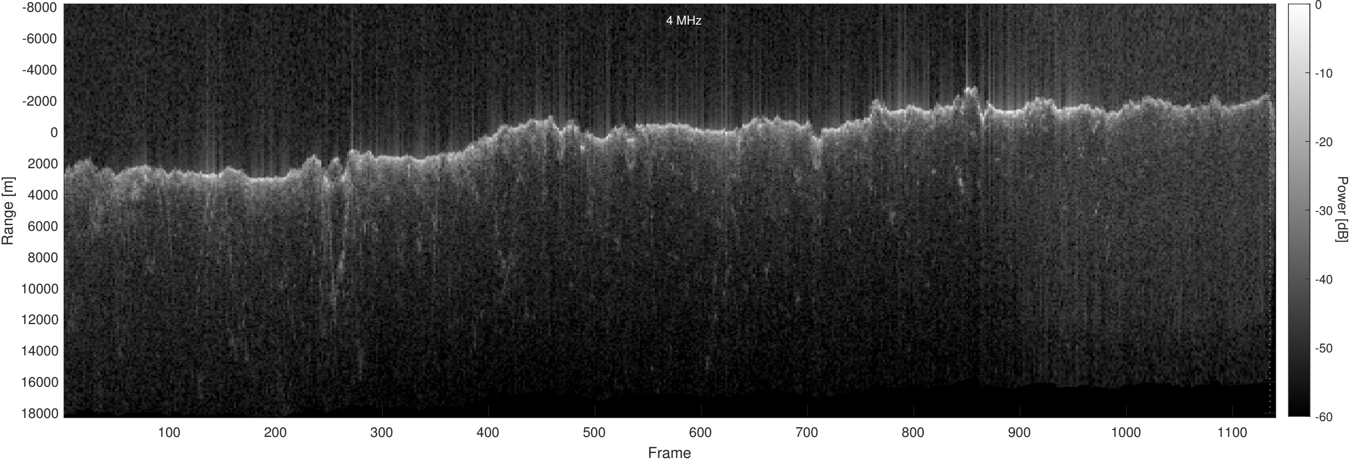
Orbit 13358, Optimized, No Window, Depth-Corrected, Channel 2
