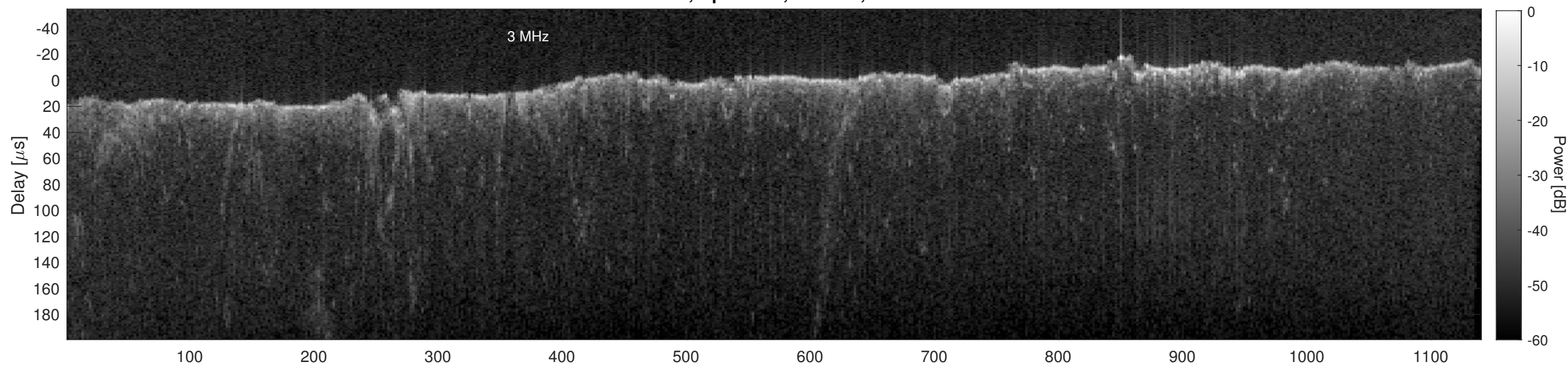
Orbit 13358, Cluttergram
