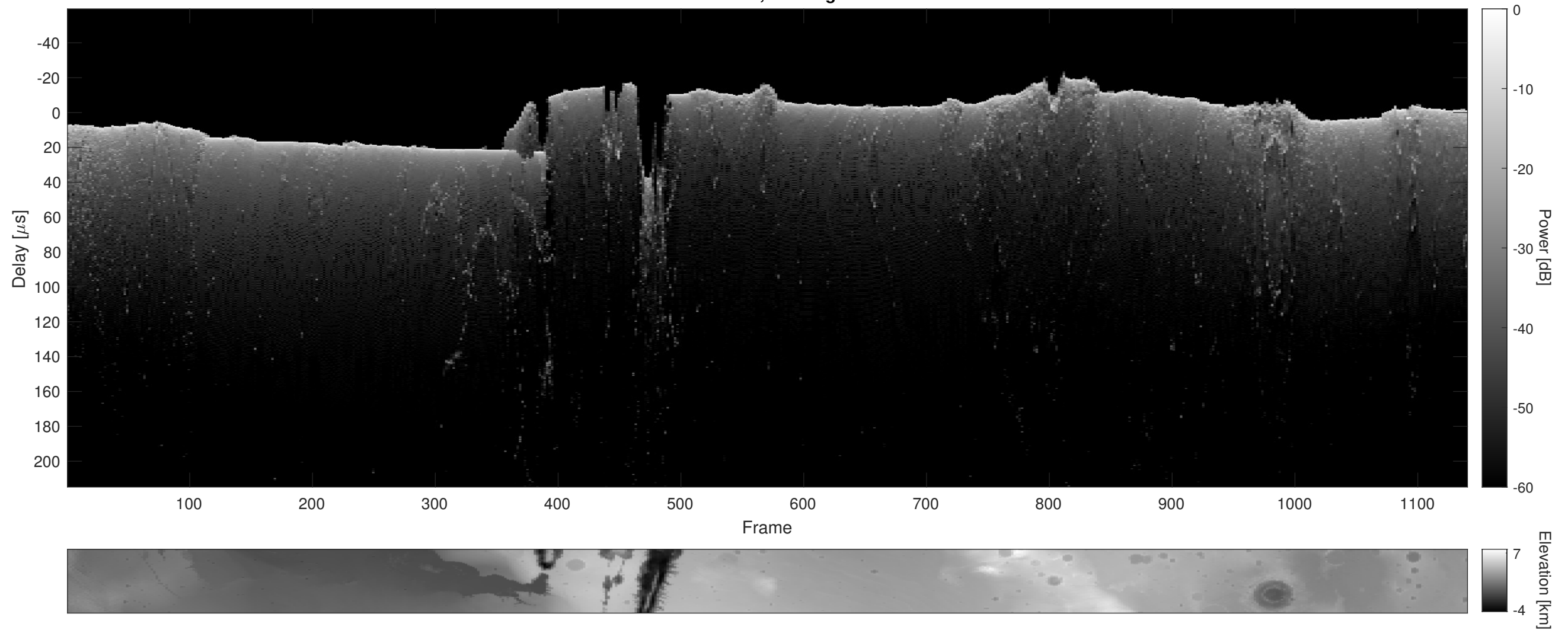
Orbit 13359, Cluttergram
