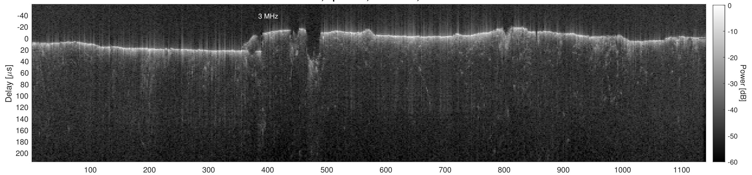
Orbit 13359, Cluttergram
