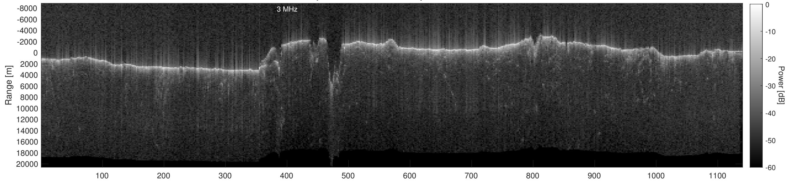
Orbit 13359, Depth-Corrected Cluttergram
