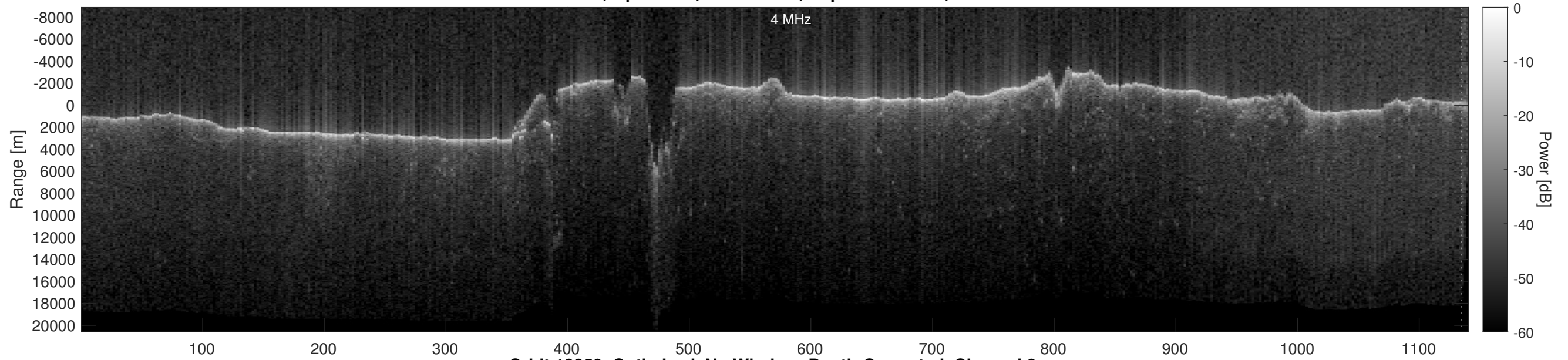
Orbit 13359, Optimized, No Window, Depth-Corrected, Channel 2
