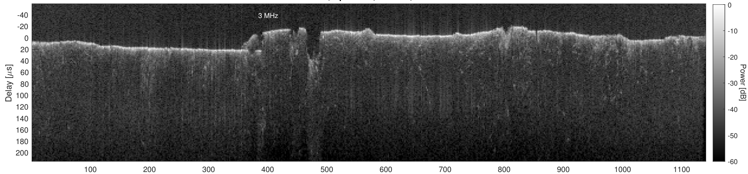
Orbit 13359, Cluttergram
