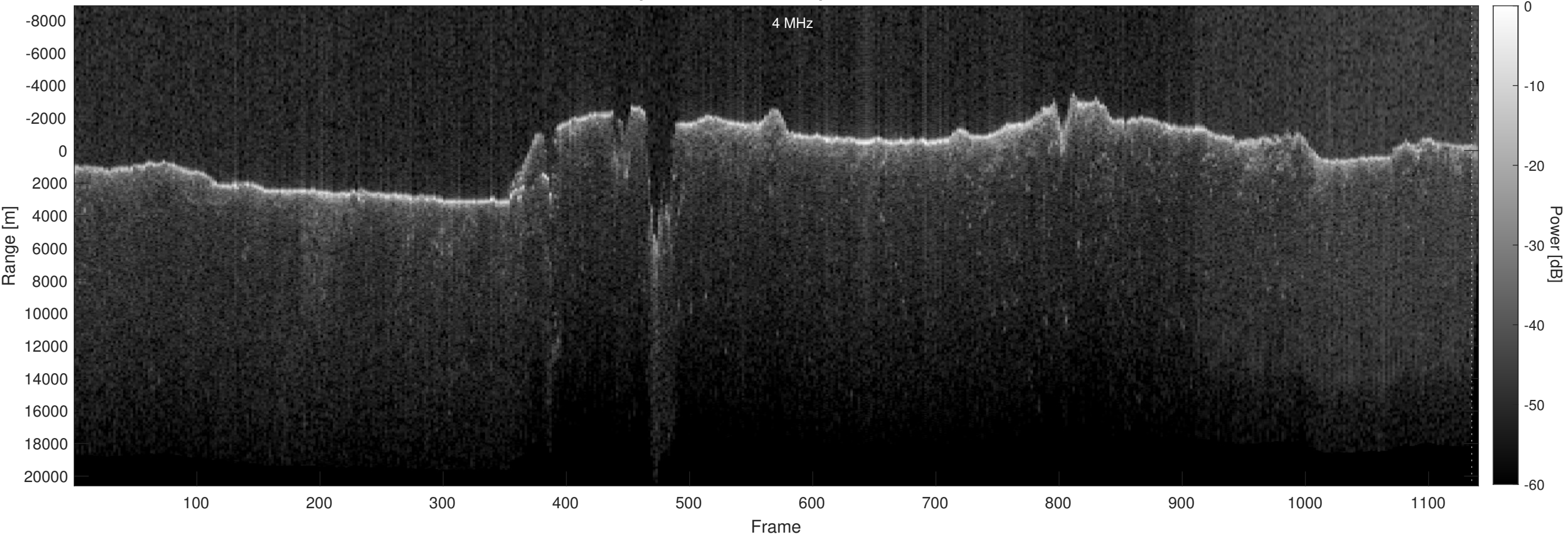
Orbit 13359, Optimized, Window, Depth-Corrected, Channel 2
