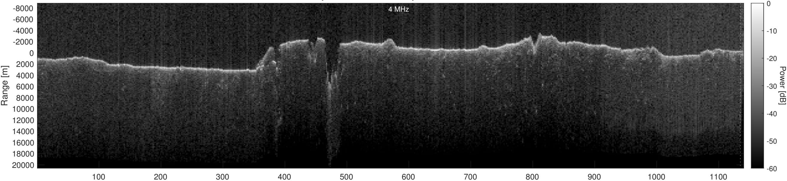
Orbit 13359, Optimized, Window, Depth-Corrected, Channel 2
