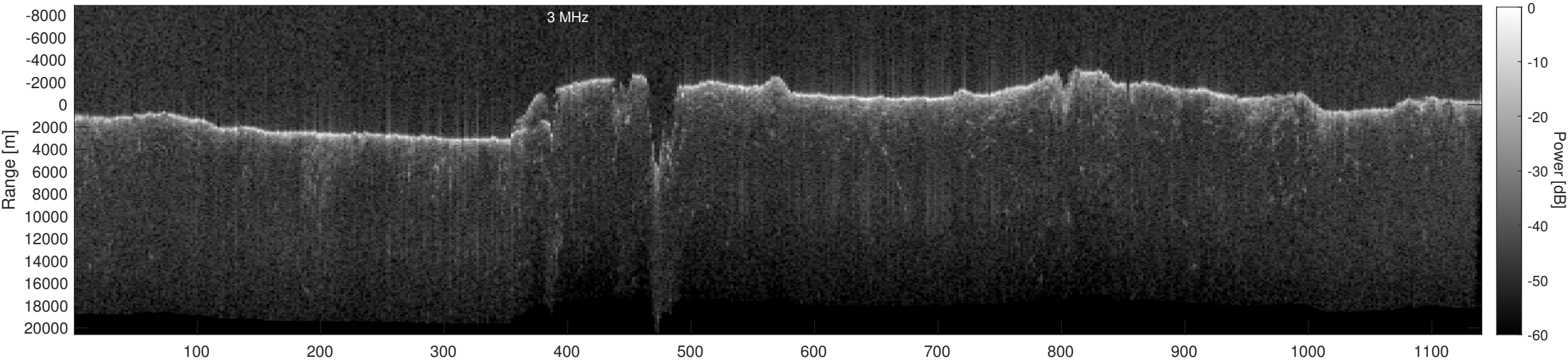
Orbit 13359, Depth-Corrected Cluttergram
