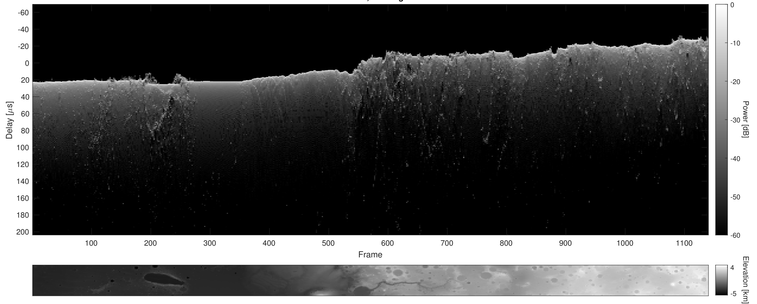
Orbit 13360, Cluttergram
