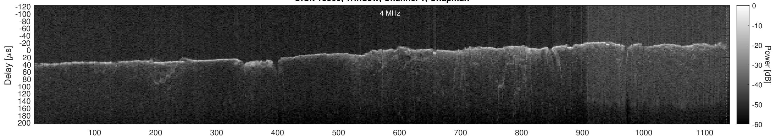
Orbit 13360, Window, Channel 1, Optimized
