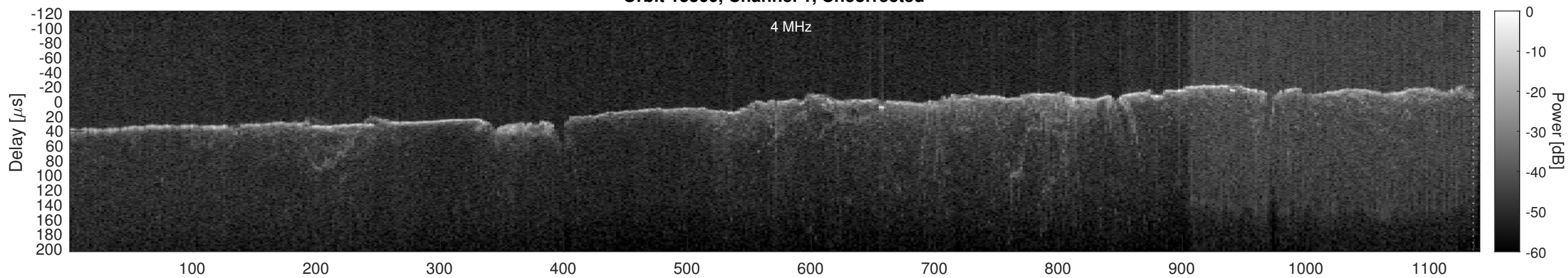
Orbit 13360, Window, Channel 1, Chapman
