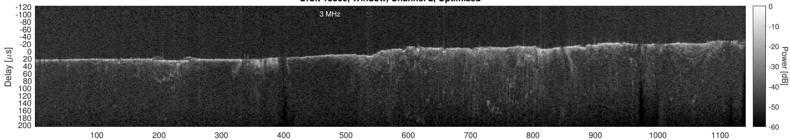
Orbit 13360, Cluttergram
