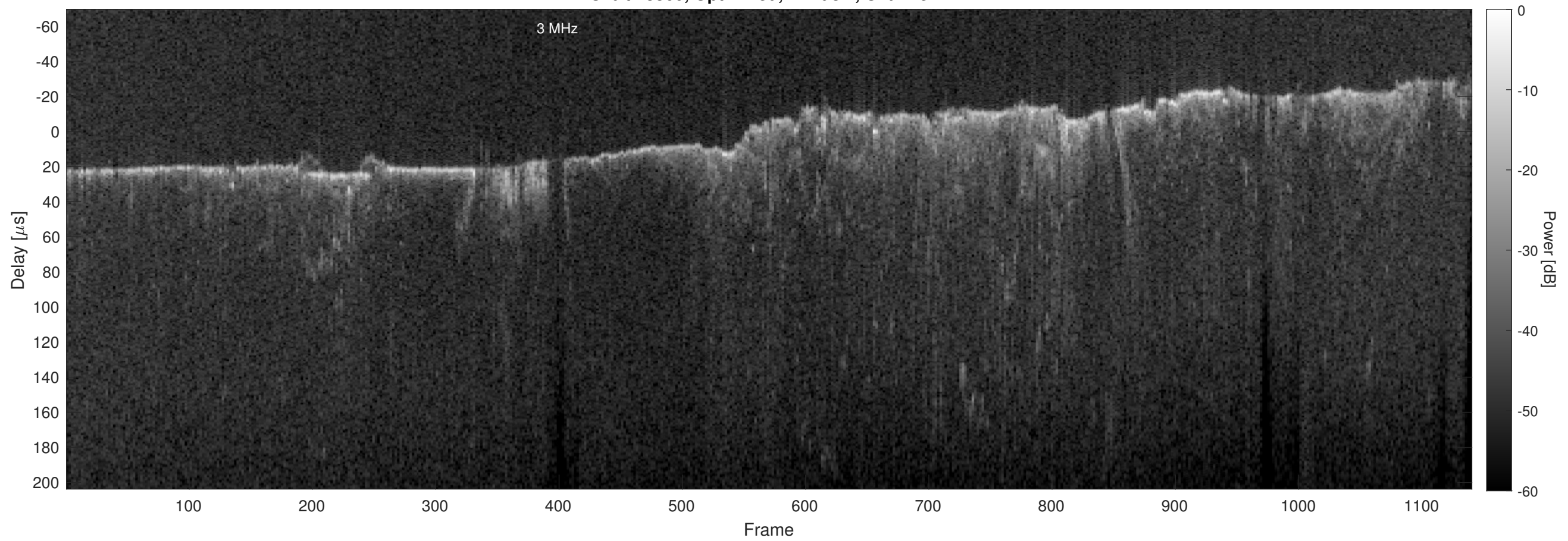
Orbit 13360, Optimized, Window, Channel 2
