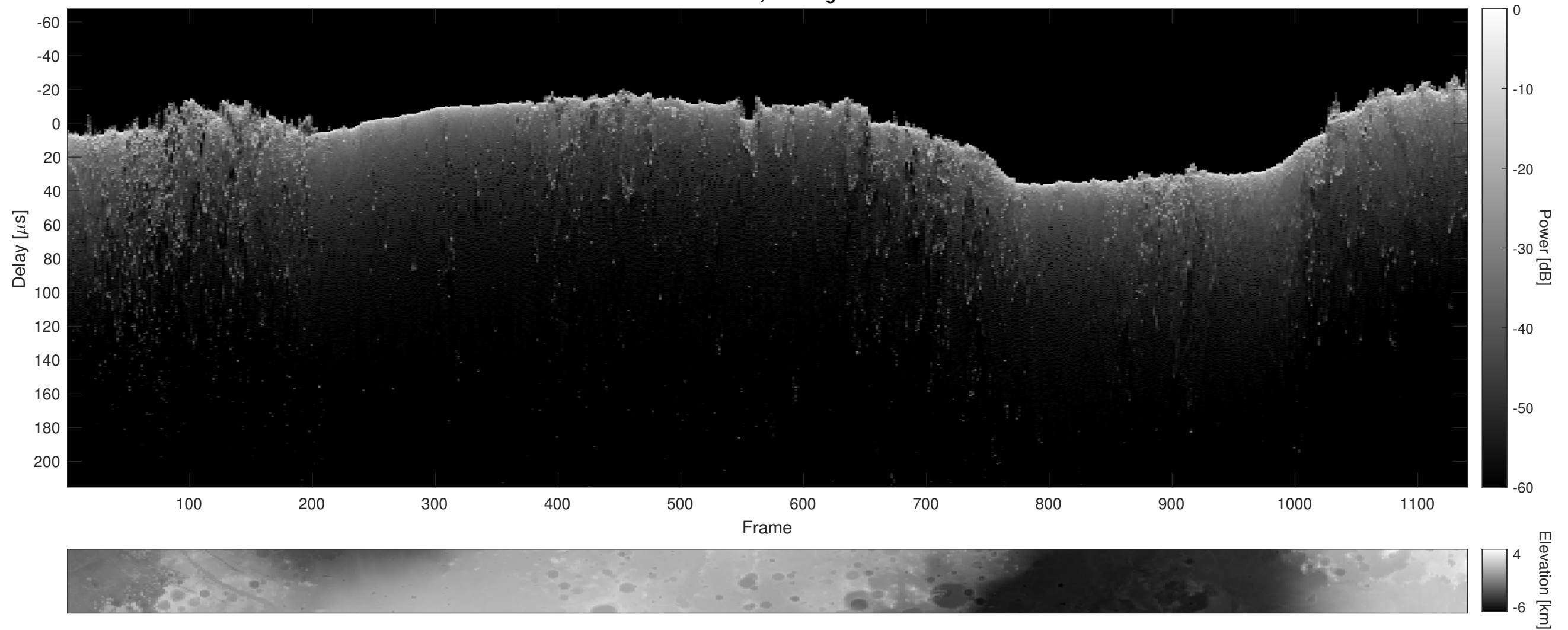
Orbit 13361, Cluttergram
