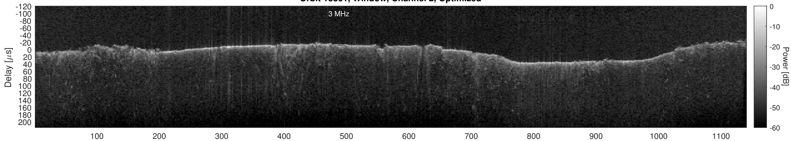
Orbit 13361, Cluttergram
