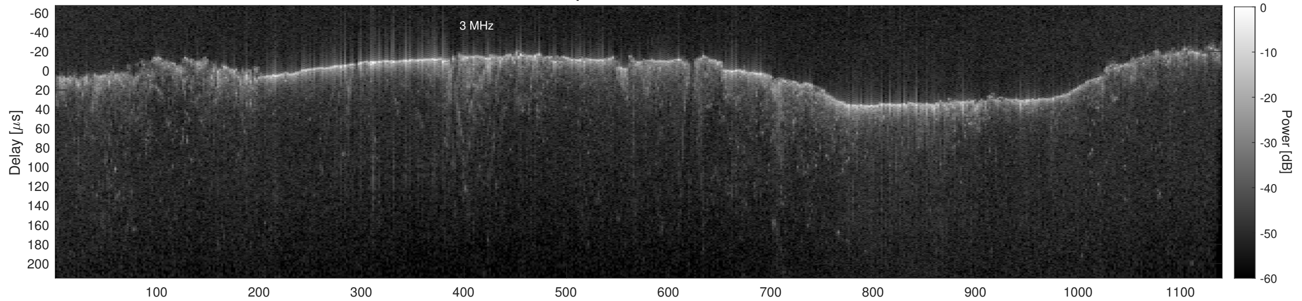
Orbit 13361, Cluttergram
