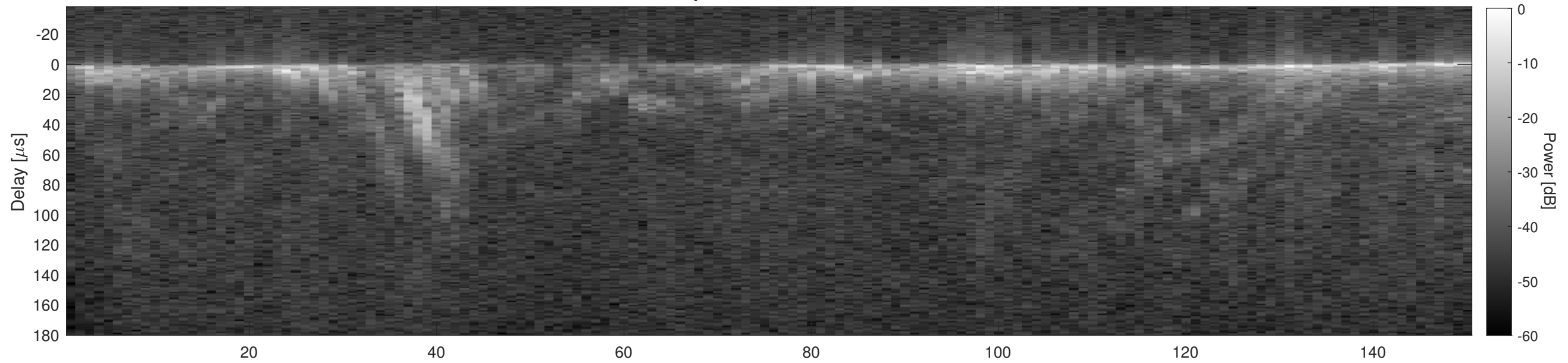
Orbit 13362, Cluttergram
