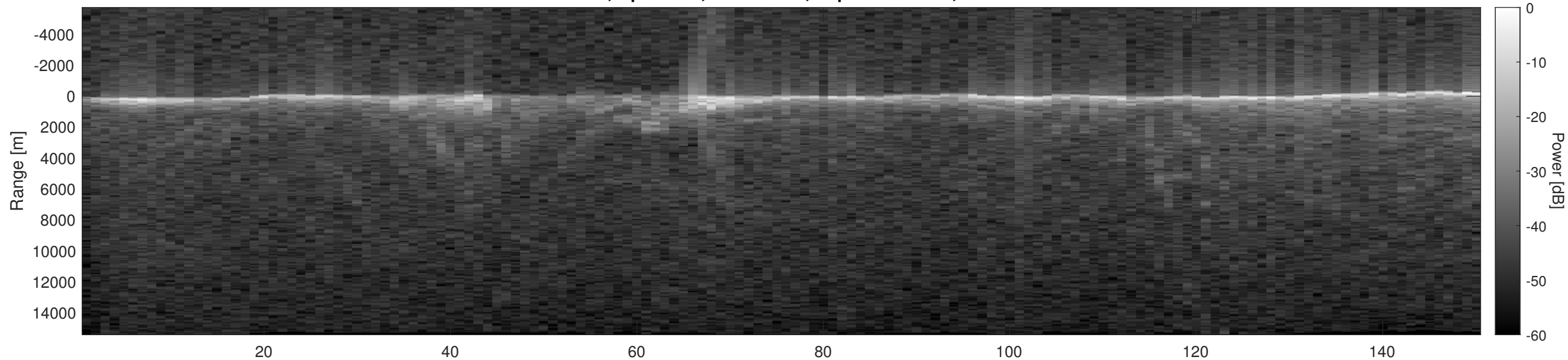
Orbit 13362, Optimized, No Window, Depth-Corrected, Channel 2
