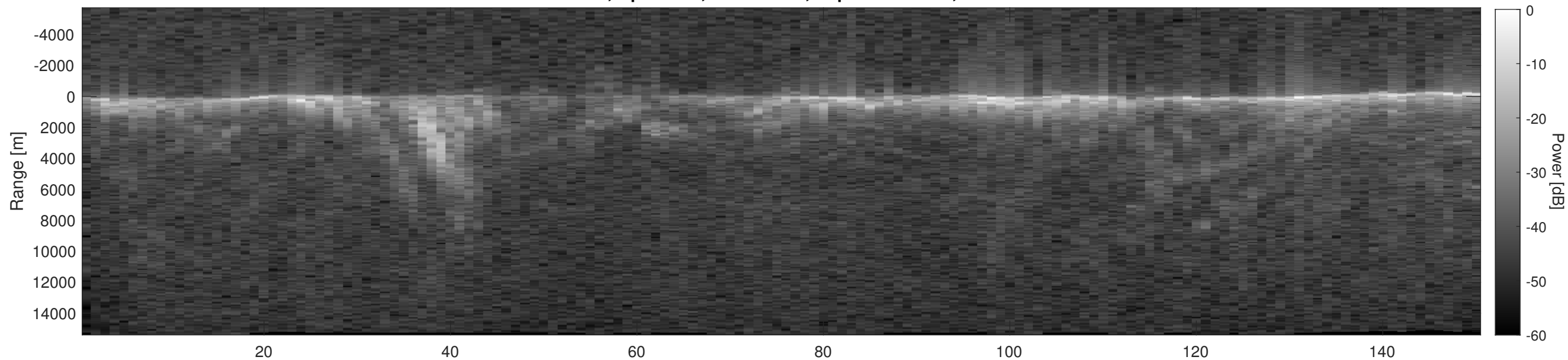
Orbit 13362, Depth-Corrected Cluttergram
