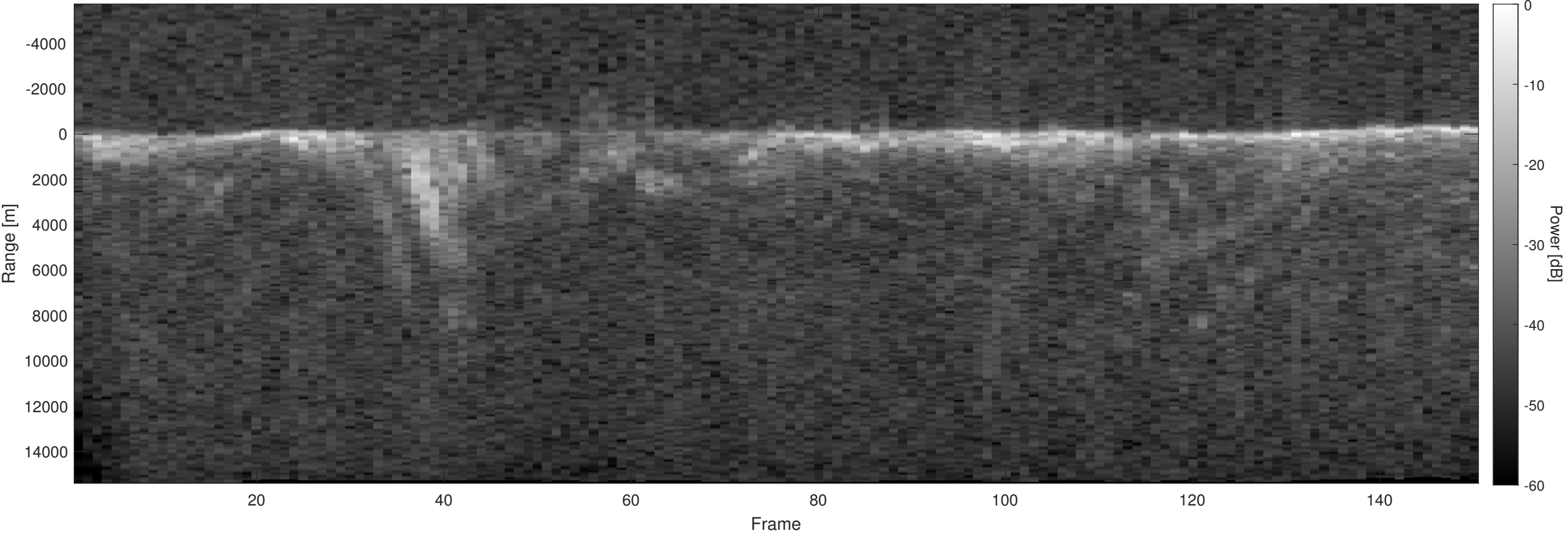
Orbit 13362, Optimized, Window, Depth-Corrected, Channel 2
