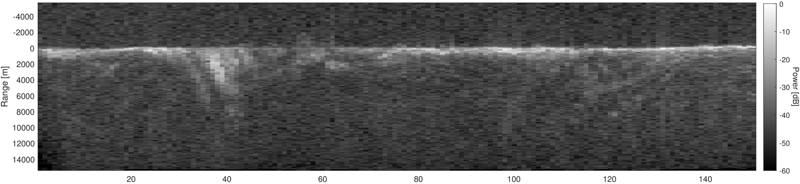
Orbit 13362, Depth-Corrected Cluttergram
