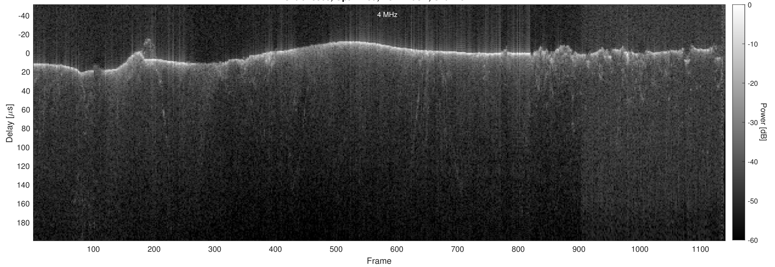
Orbit 13363, Optimized, No Window, Channel 2
