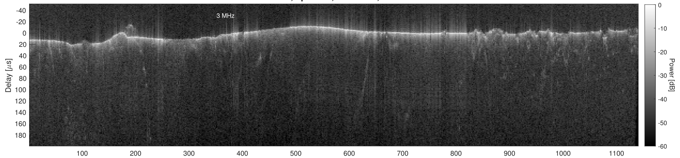
Orbit 13363, Cluttergram
