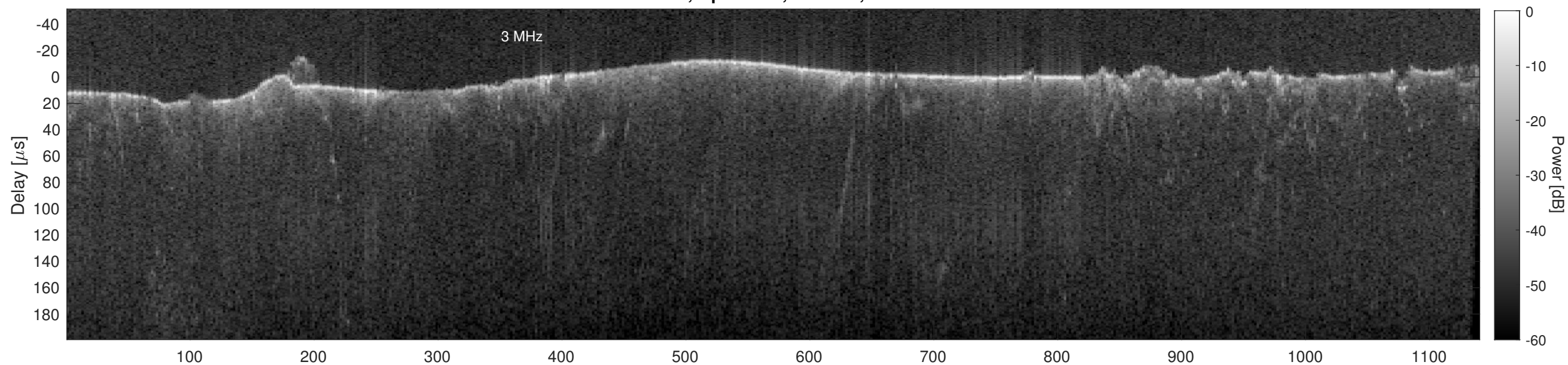
Orbit 13363, Cluttergram
