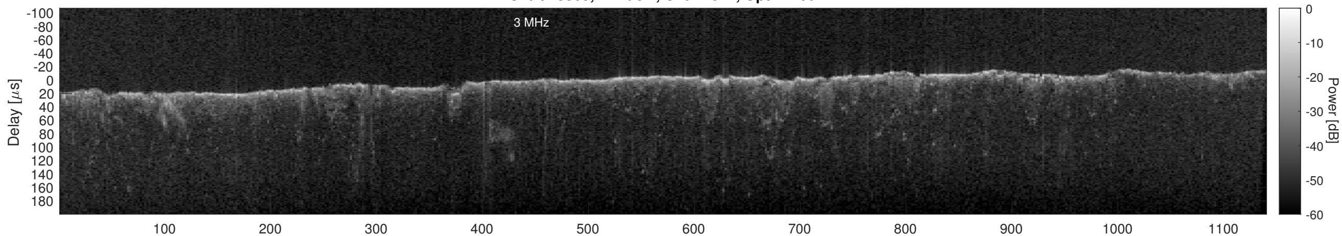
Orbit 13365, Cluttergram
