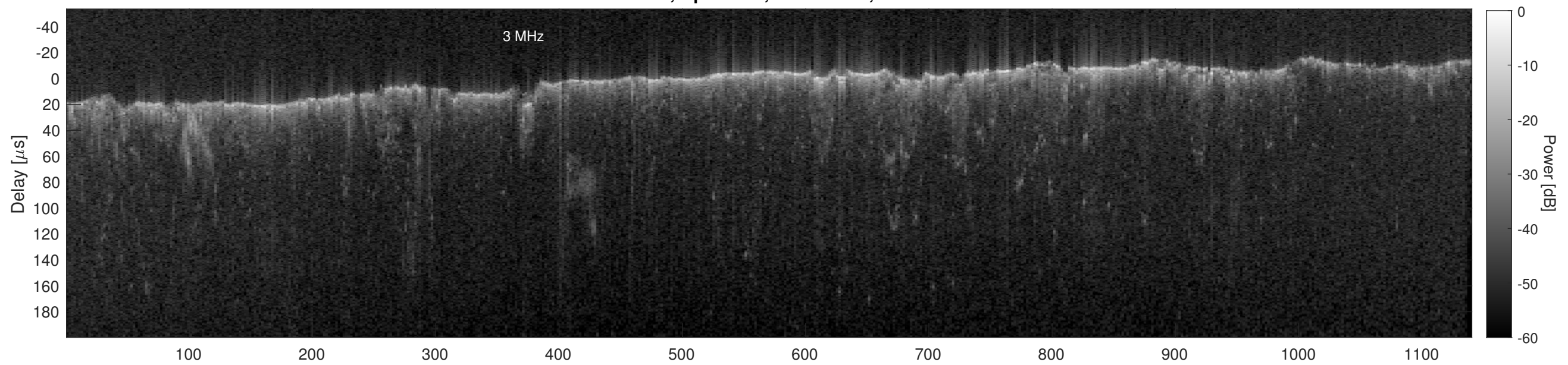
Orbit 13365, Cluttergram
