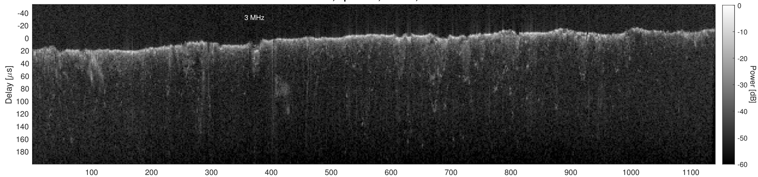
Orbit 13365, Cluttergram
