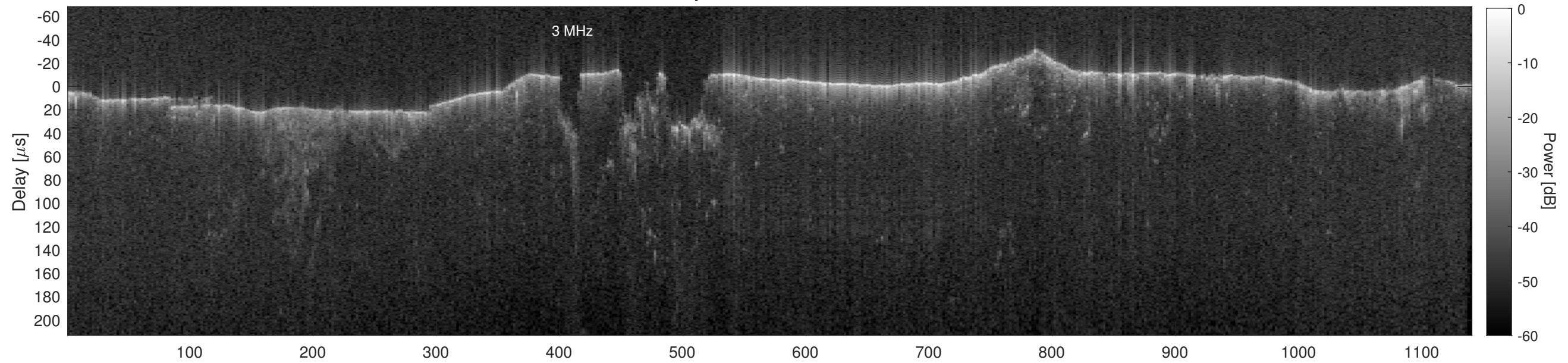
Orbit 13366, Cluttergram
