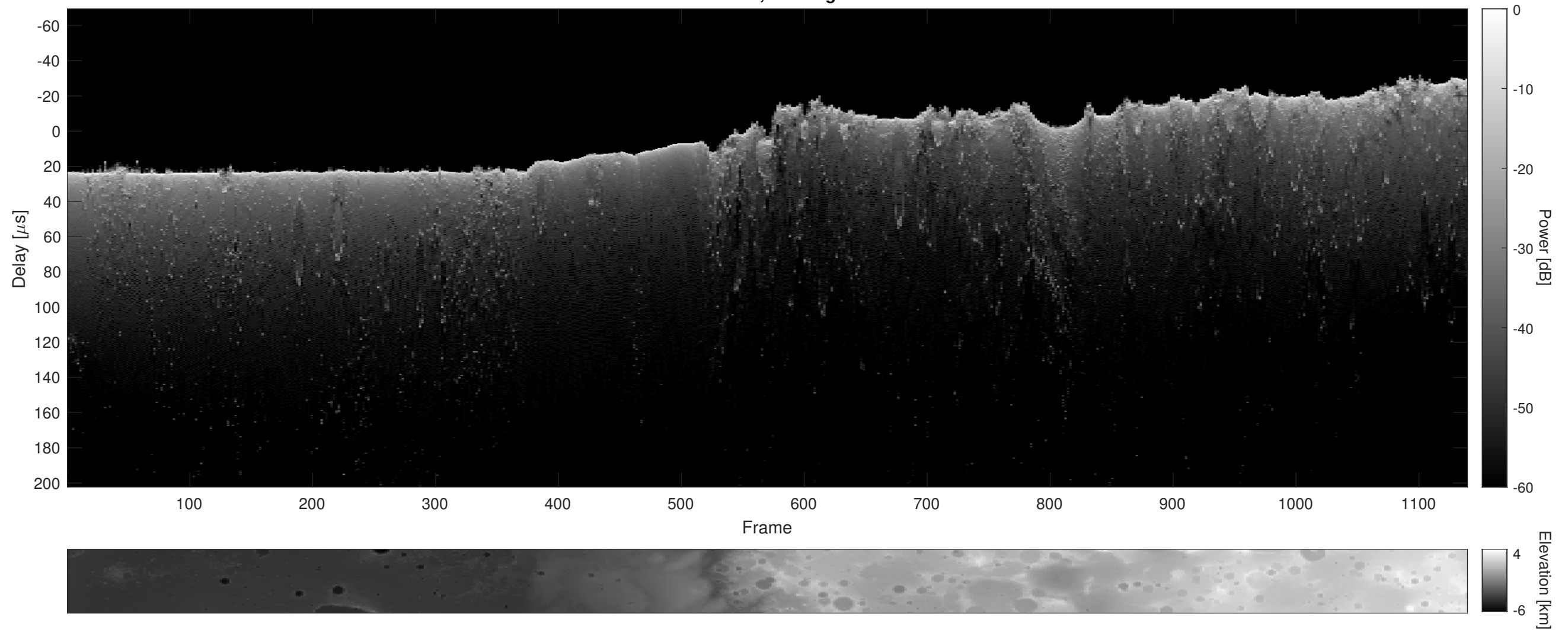
Orbit 13367, Cluttergram
