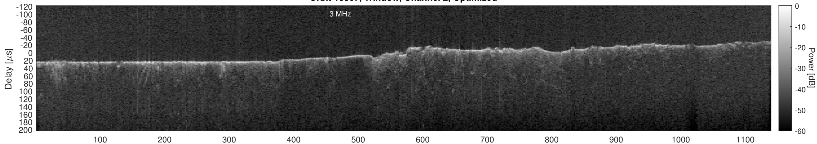
Orbit 13367, Cluttergram
