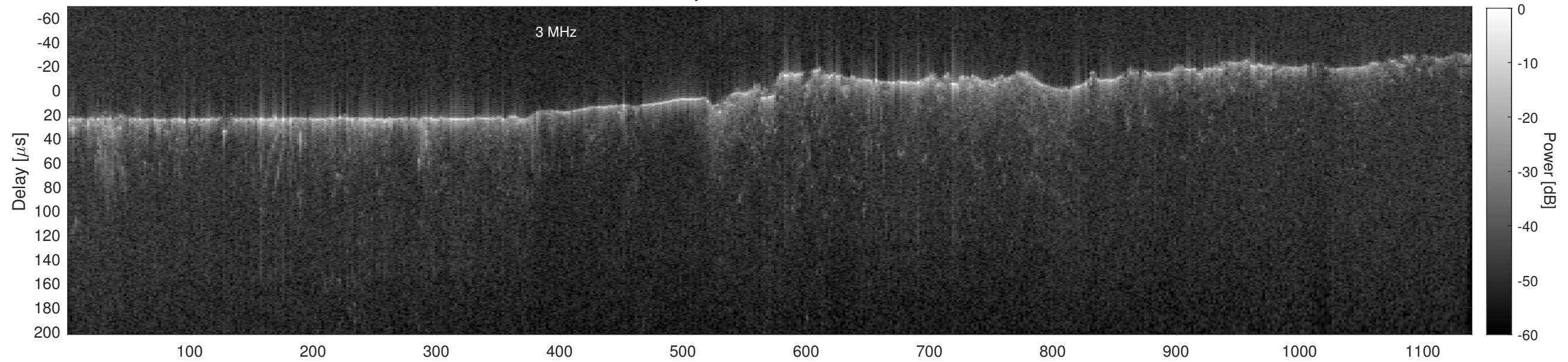
Orbit 13367, Cluttergram
