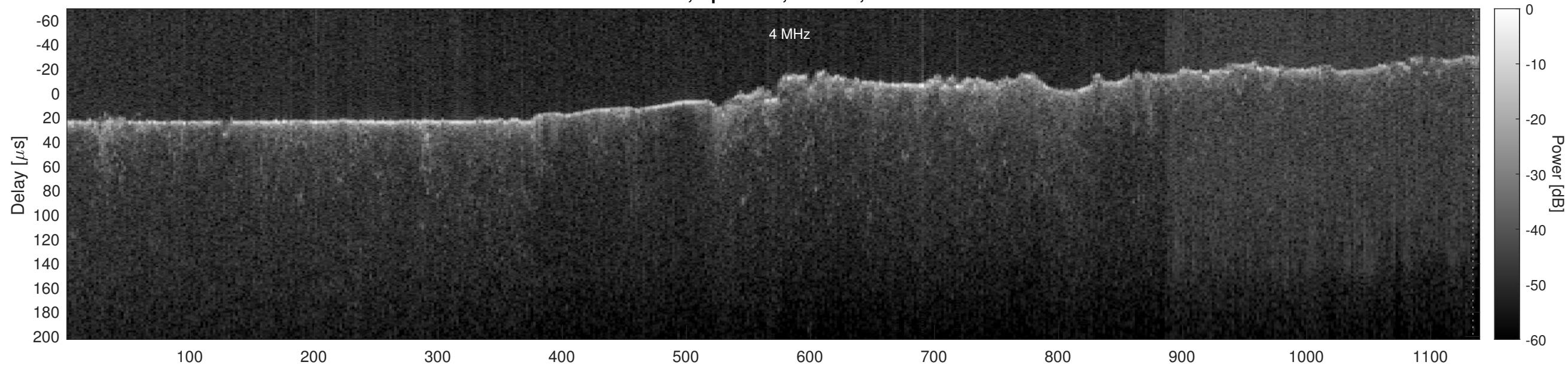
Orbit 13367, Optimized, Window, Channel 2
