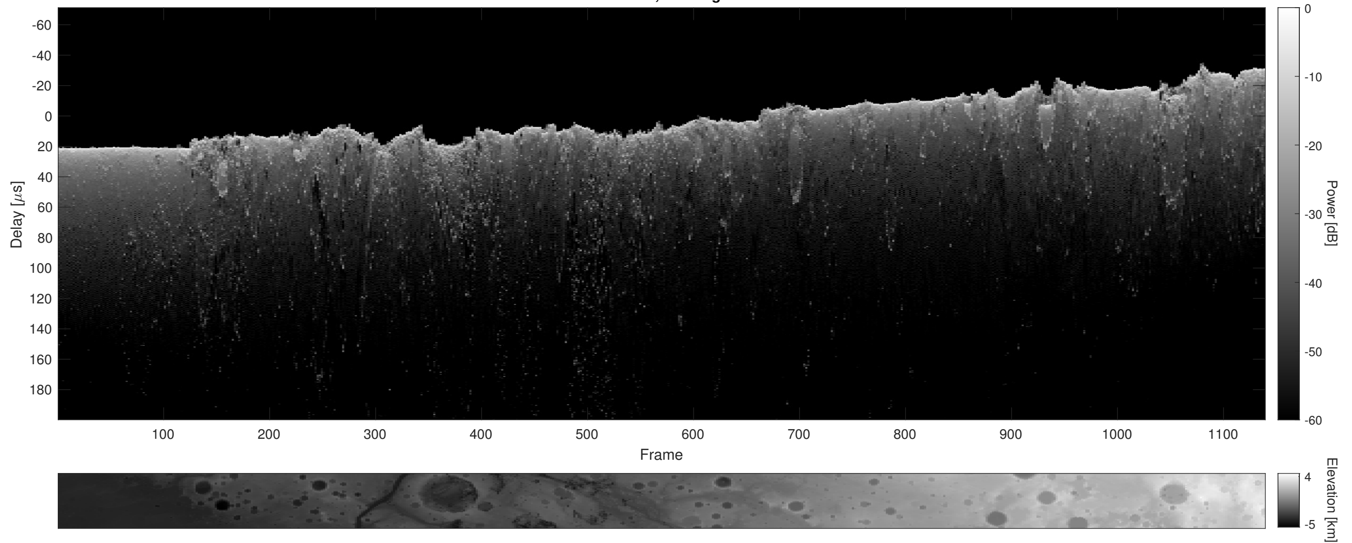
Orbit 13369, Cluttergram
