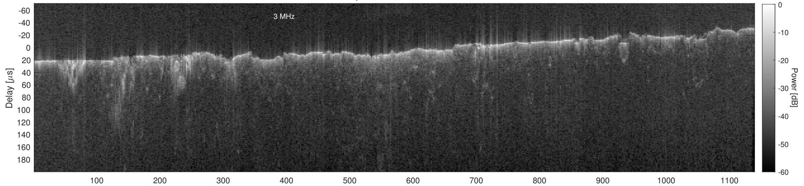
Orbit 13369, Cluttergram
