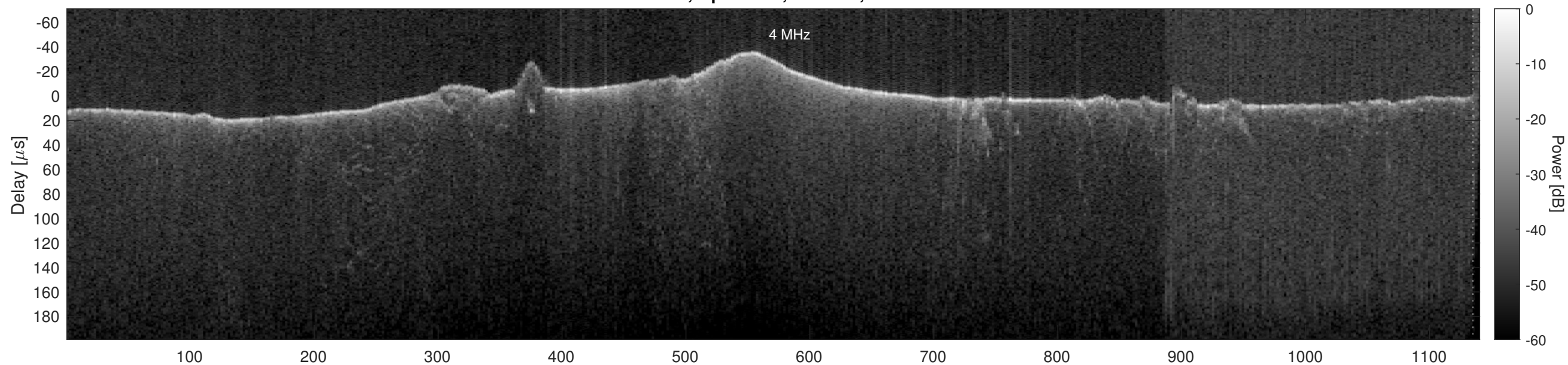
Orbit 13370, Optimized, Window, Channel 2
