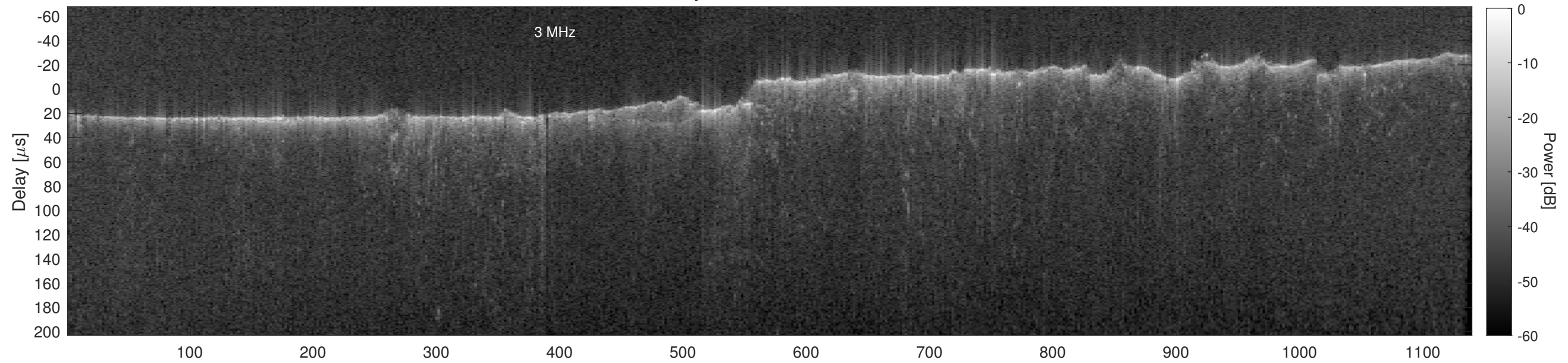
Orbit 13374, Cluttergram
