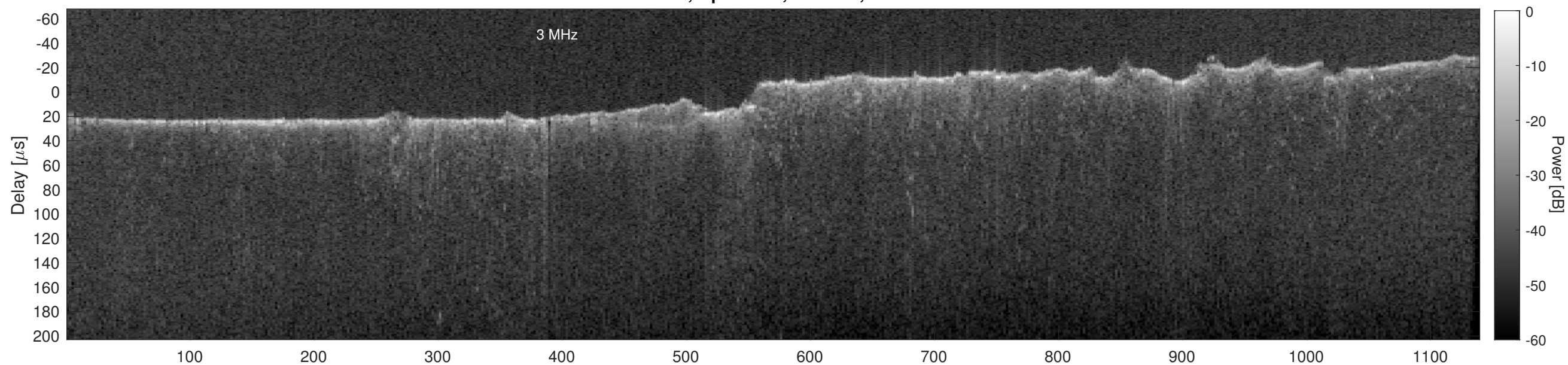
Orbit 13374, Cluttergram
