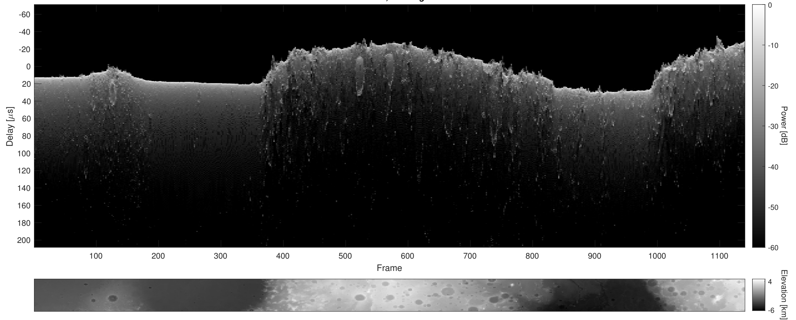
Orbit 13375, Cluttergram
