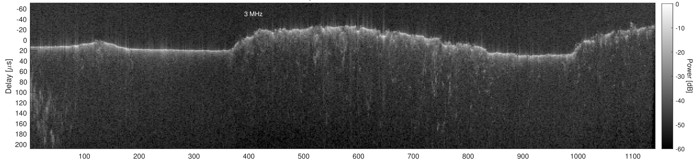
Orbit 13375, Cluttergram
