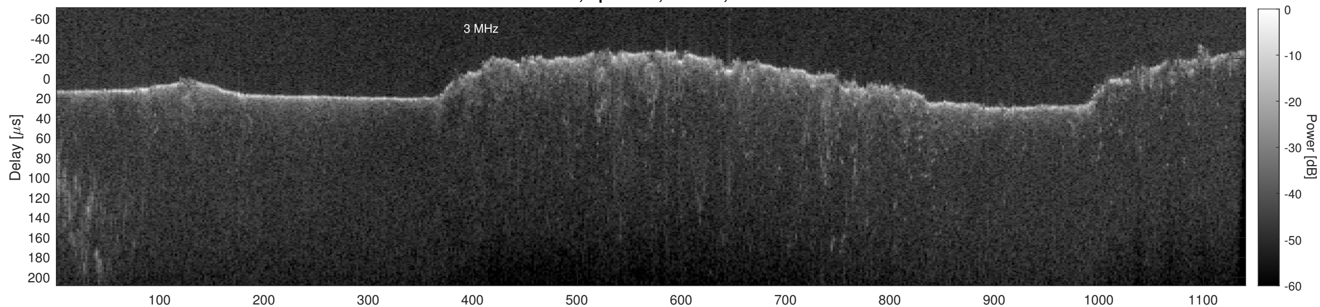
Orbit 13375, Cluttergram
