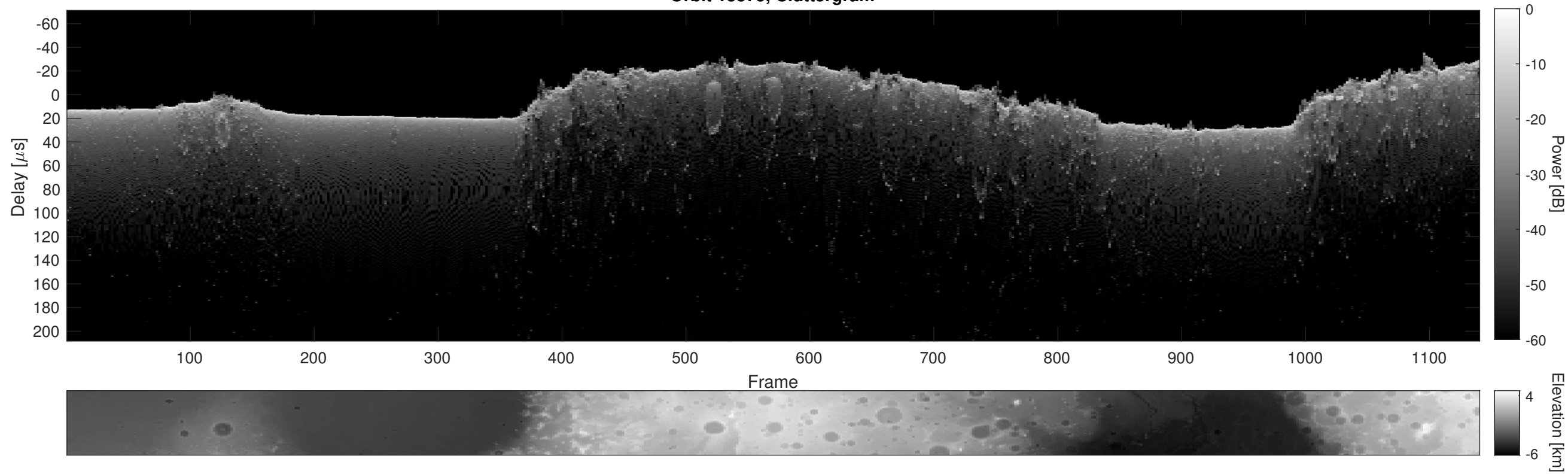
Orbit 13375, Cluttergram
