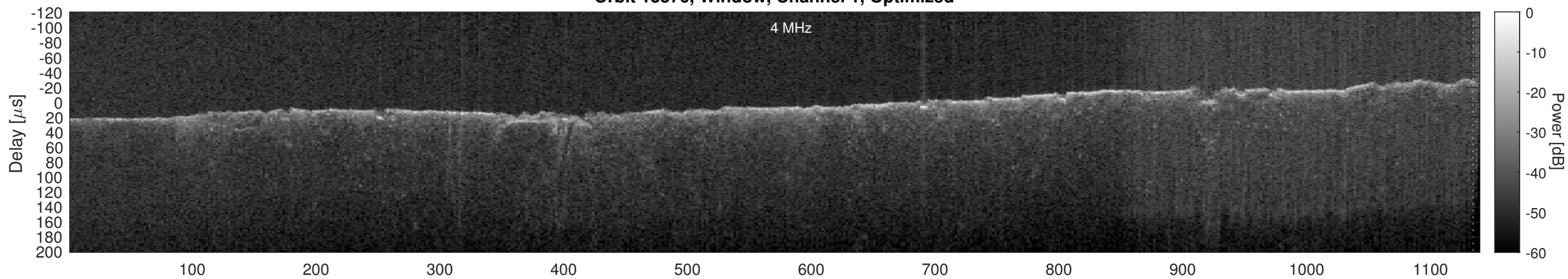
Orbit 13376, Cluttergram
