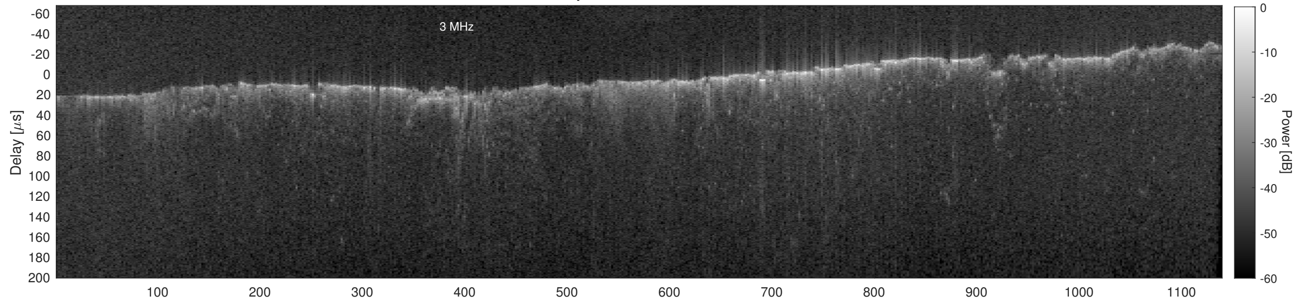
Orbit 13376, Cluttergram
