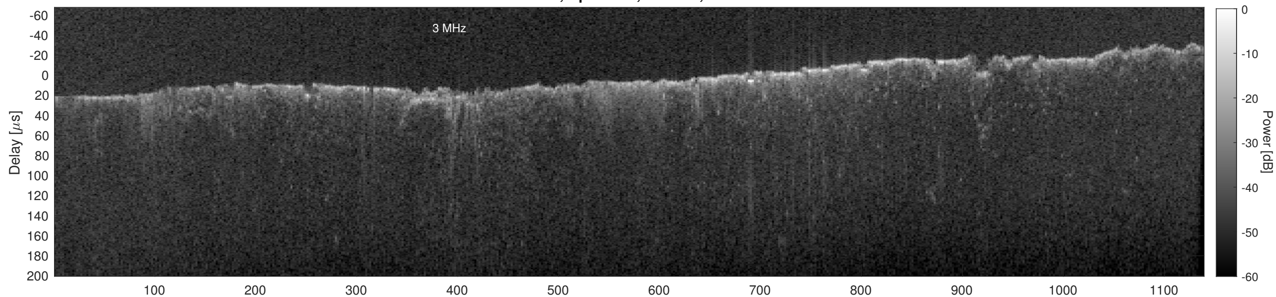
Orbit 13376, Cluttergram
