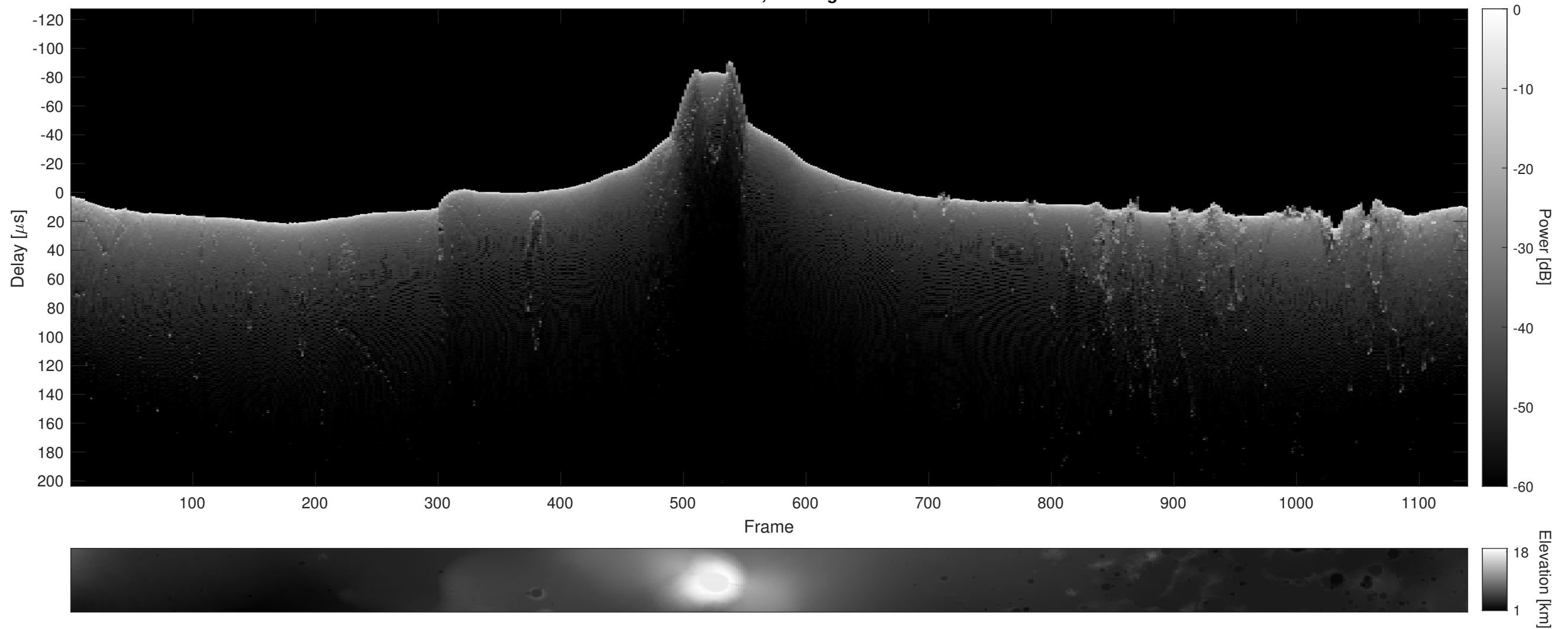
Orbit 13377, Cluttergram
