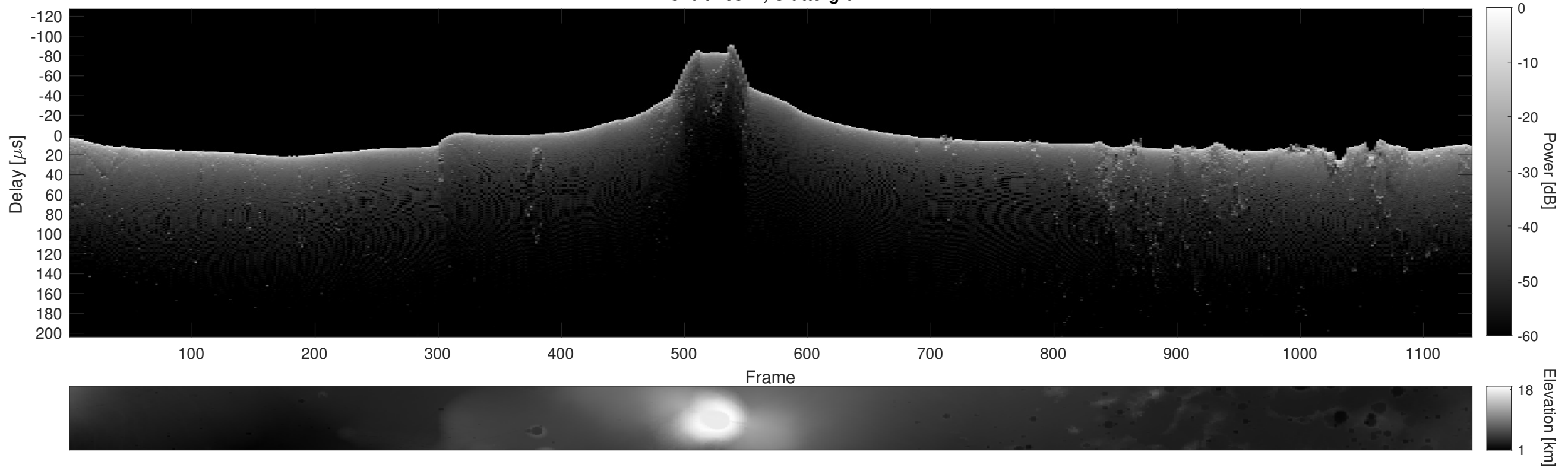
Orbit 13377, Cluttergram
