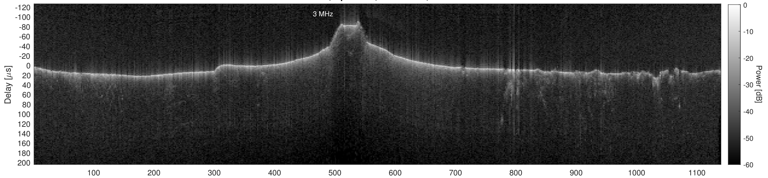
Orbit 13377, Cluttergram
