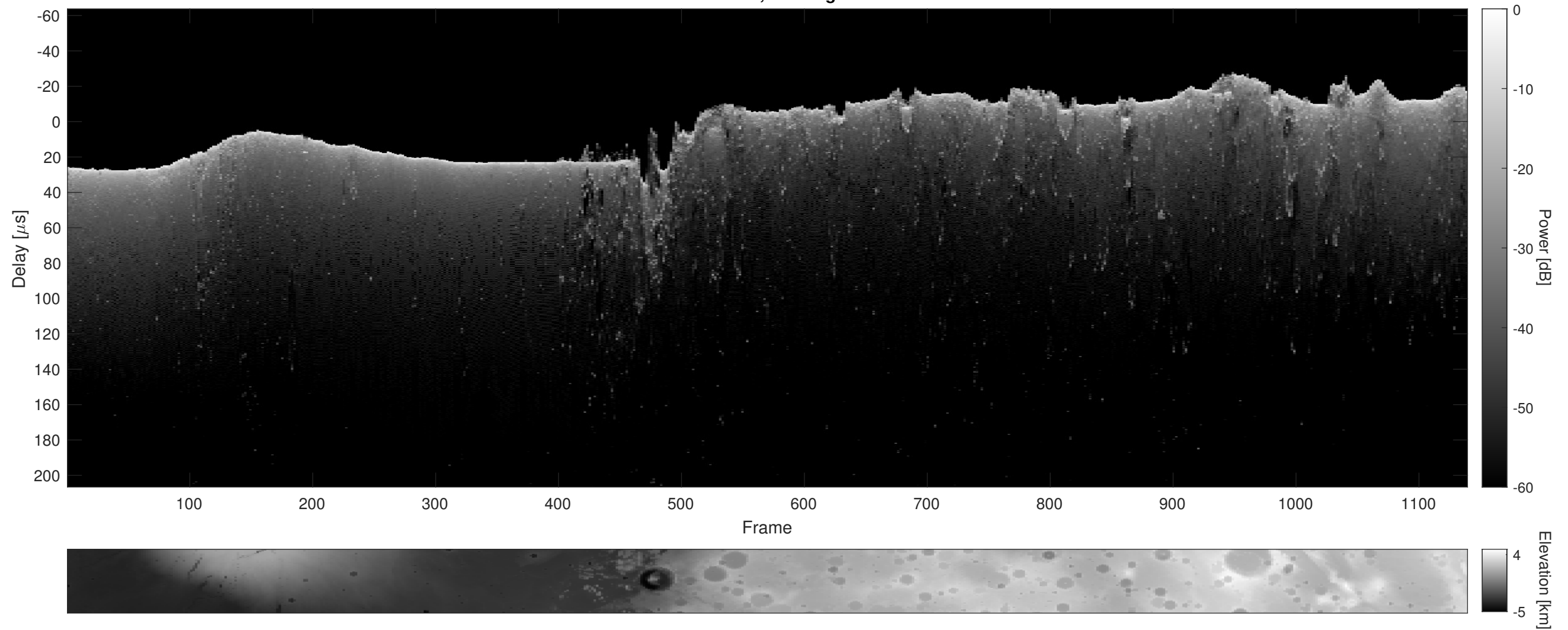
Orbit 13378, Cluttergram
