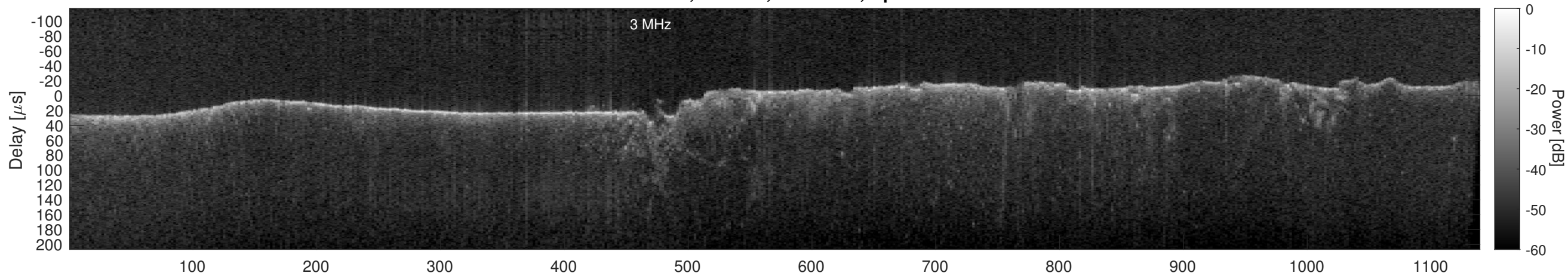
Orbit 13378, Cluttergram
