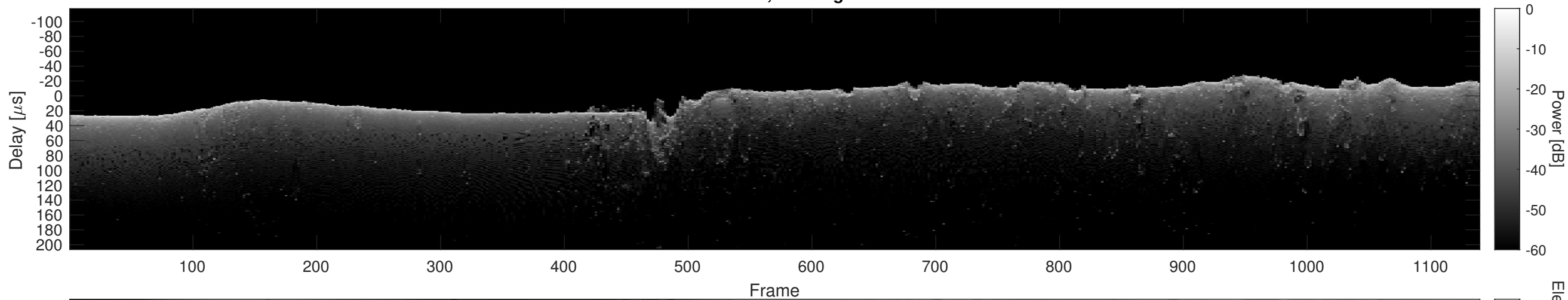
Orbit 13378, Cluttergram
